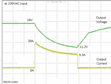
Peak load 20A (resistive) for 5 ms Output voltage dips from 24V to 11.2V
